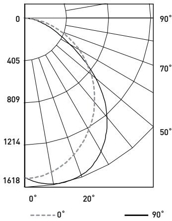
ST3-**-04-H-30K-W-**** Initial Delivered Lumens: 3,600
