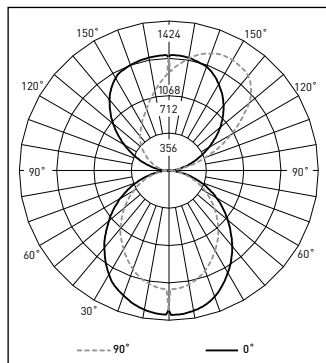
ST3-WI-04-H-H-30K-L-**** Initial Delivered Lumens: 6,624
