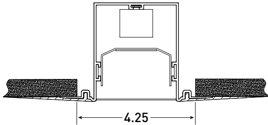
Hard Ceiling Flanegless
